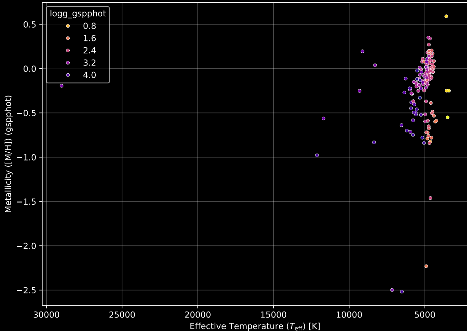
APOGEE DR17 Field: [K2_C7_010-10_btx] Stellar Population Parameters (n= 169)
