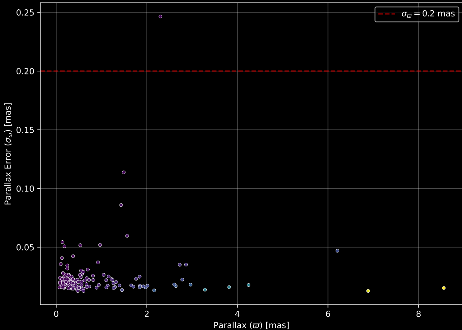
APOGEE DR17 Field: [K2_C7_010-10_btx] Parallax Quality (n= 169)
