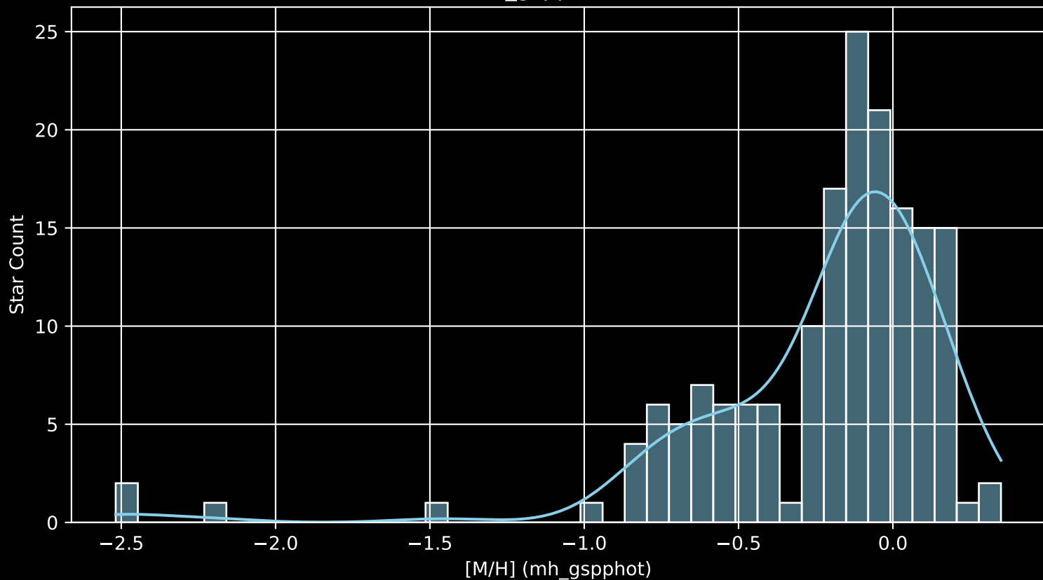
APOGEE DR17 Field: [K2_C7_010-10_btx [M/H] (mh_gspphot) (n= 168)
