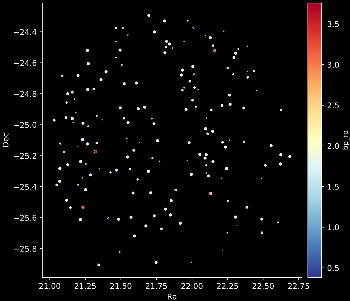
APOGEE DR17 Field: [K2_C7_010-10_btx] Stars: 169
