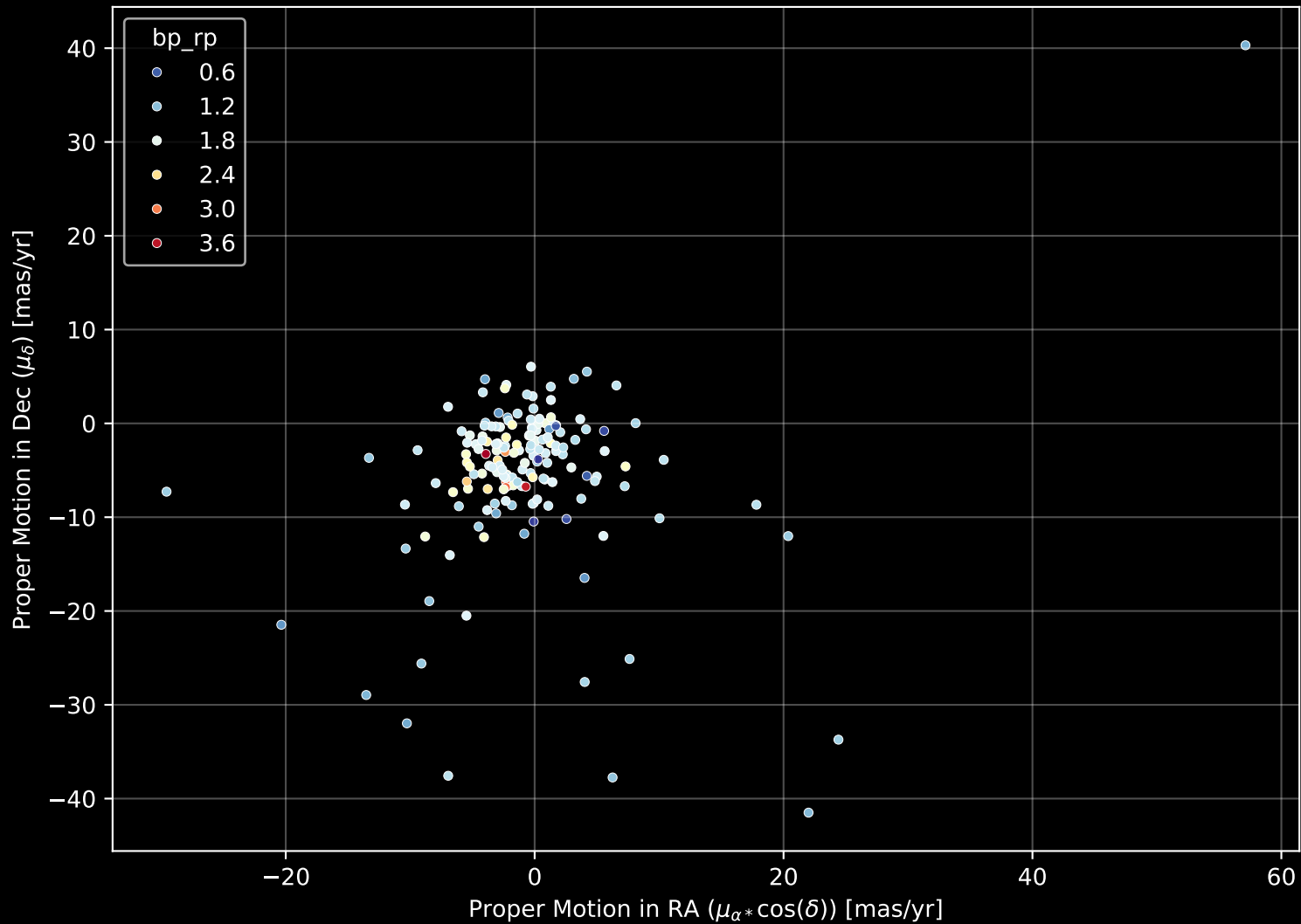
APOGEE DR17 Field: [K2_C7_010-10_btx] Proper Motion Diagram (n= 169)
