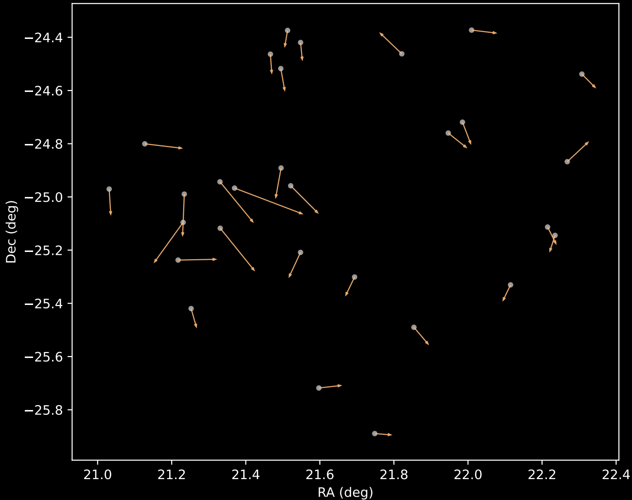
APOGEE DR17 Cluster 3 Proper Motion Vectors (n=29)
