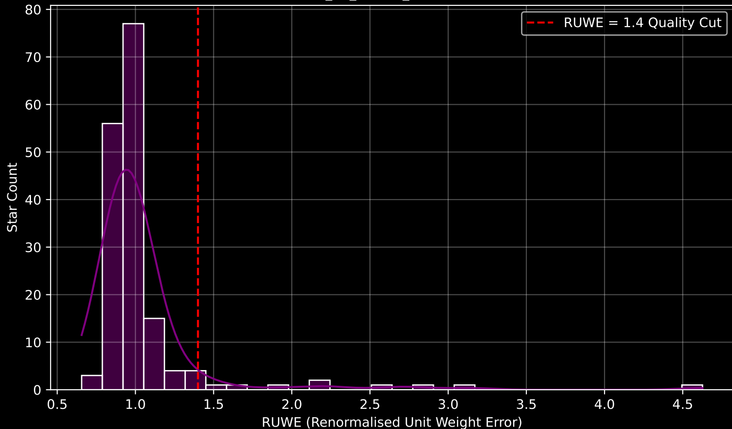
GAPOGEE DR17 Field [K2_C7_010-10_btx] RUWE Distribution (n= 168)
